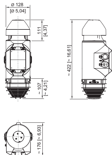
YL60/3 Cornet omnidirectionnel
