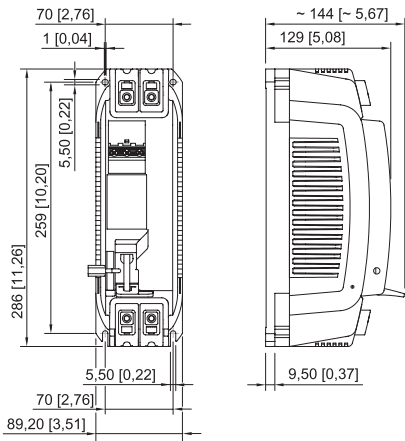
8568/MCCB, 2 pôles
