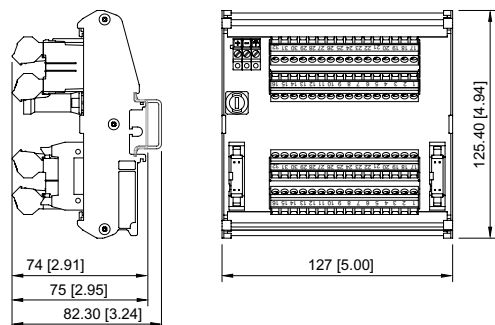
HART Termination board Type 9196/16H-XX0-05c
