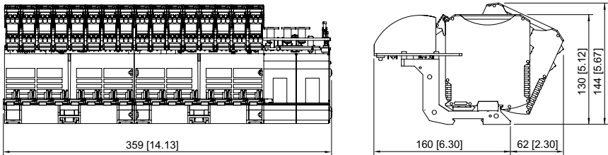
9419/08R bus-Carrier for 16 fieldbus segments
