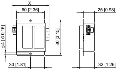
Dimensional Drawings (All Dimensions in mm [inches]) – Subject to Alterations
