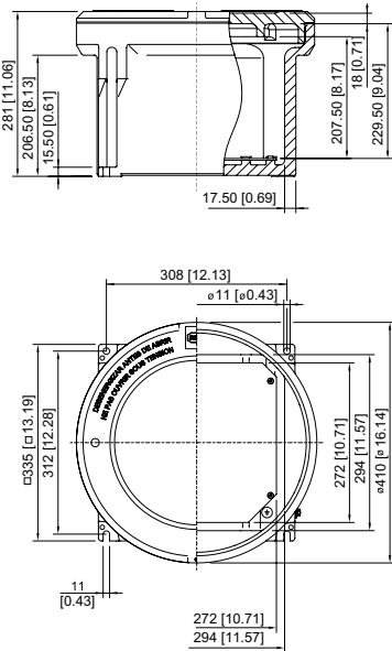
Enclosure size 6 without inspection window
