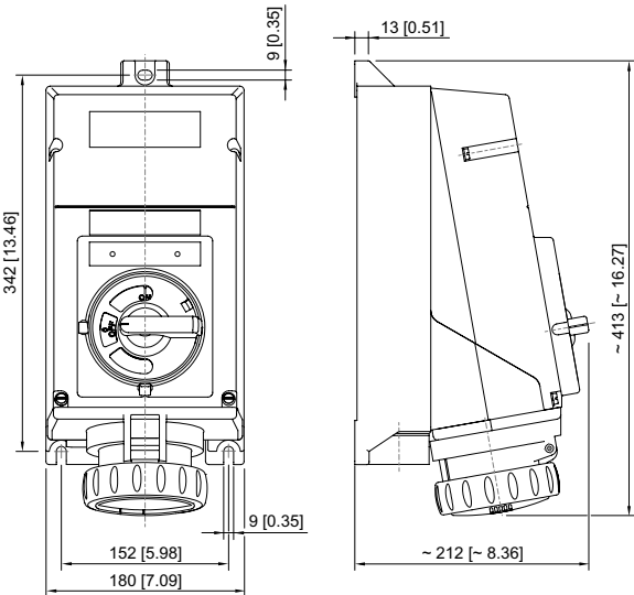
Wall-mounting receptacle
