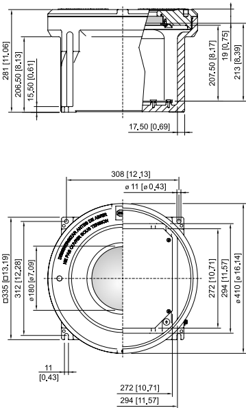
Enclosure size 6 with inspection window
