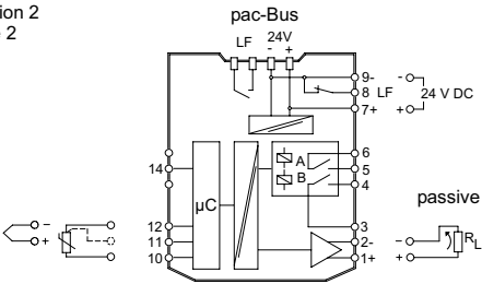
Connection diagram 9182/10-51-64
