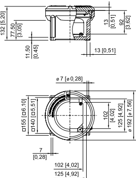
Enclosure size 2 without inspection window
