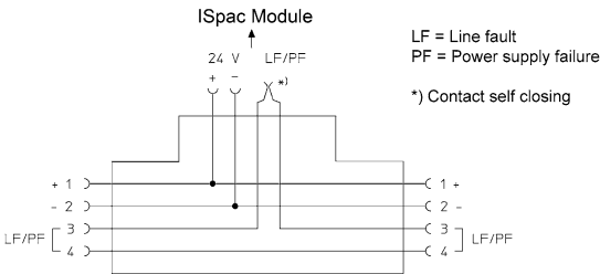
Connection Diagram 9194/50-01
