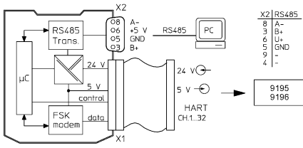
Connection Diagram 9192/32-10-10
