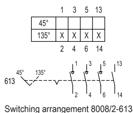
Switching arrangement 8008/2-613
