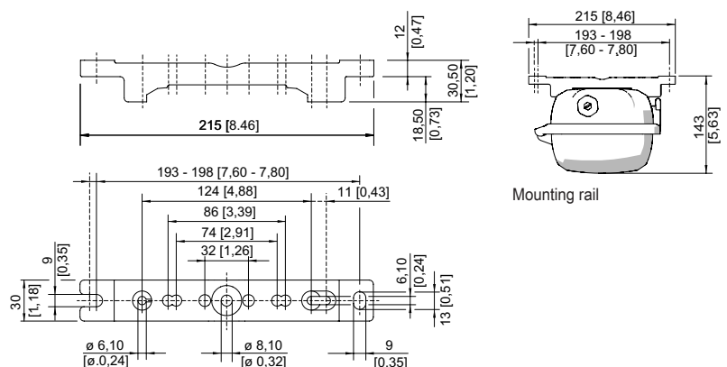
Mounting rail
