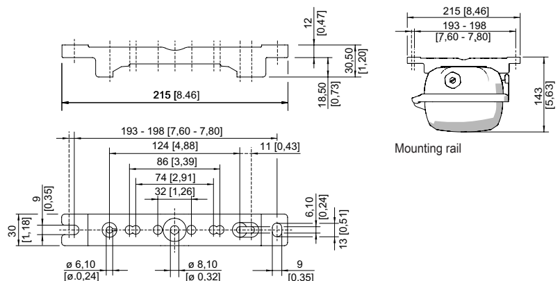
Mounting rail
