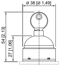
8003/...-008 key-operated switch
