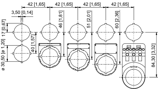
8003/...-008 key-operated switch
