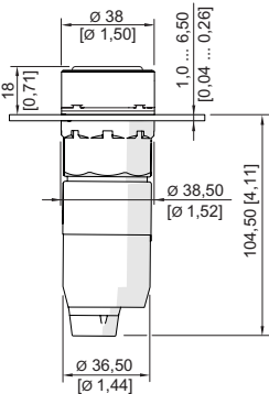
LED illuminated pushbutton
