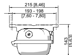
Mounting rail
