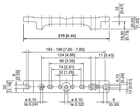
Mounting rail
