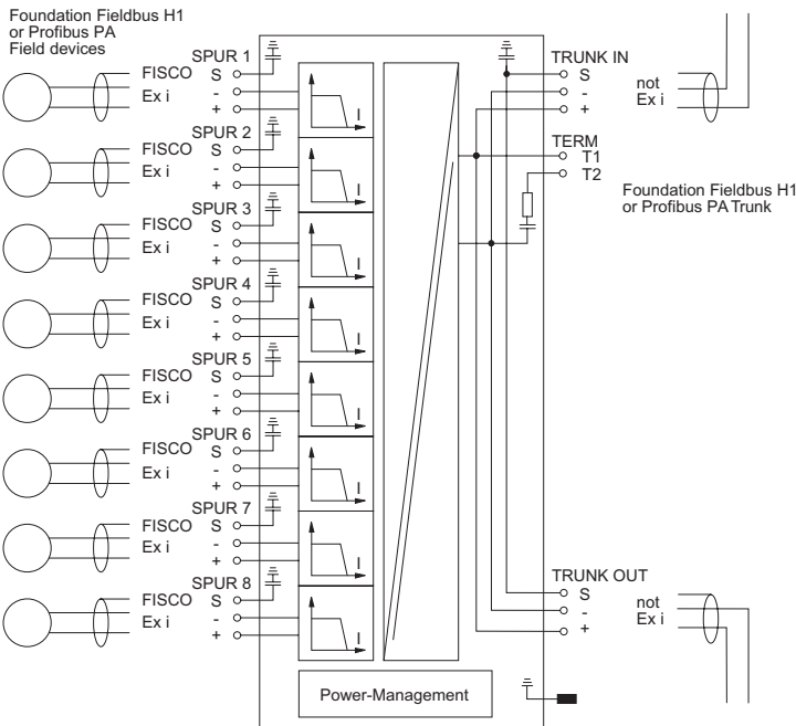
Connection diagram 9411/2.
