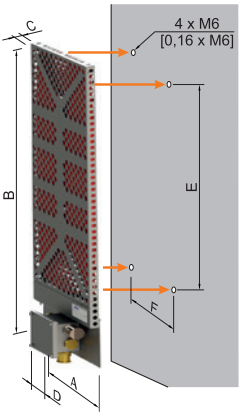
Note! Never install the heater with junction box facing upwards.
