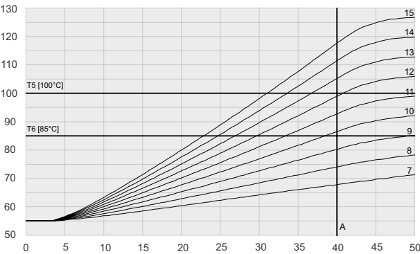
8405/6-1T-5-Ta = 55°C
