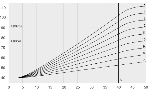
8405/6-1T-5-Ta = 50°C
