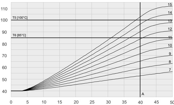
8405/6-1T-5-Ta = 40°C
