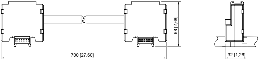
BusRail extension
