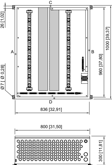
1 x BusRail for 16 slots
