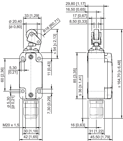
Roller lever 8070/2-3-WH-U60
