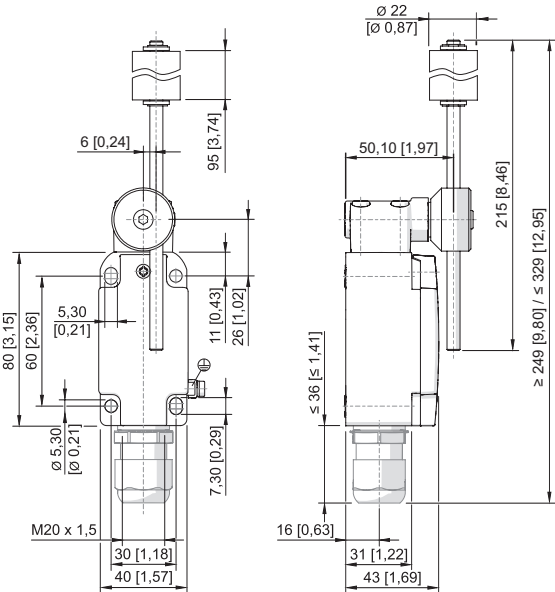
Misalignment switch 8074/2-.-SR-40
