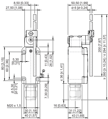
Rod lever 8074/2-2-DD-40
