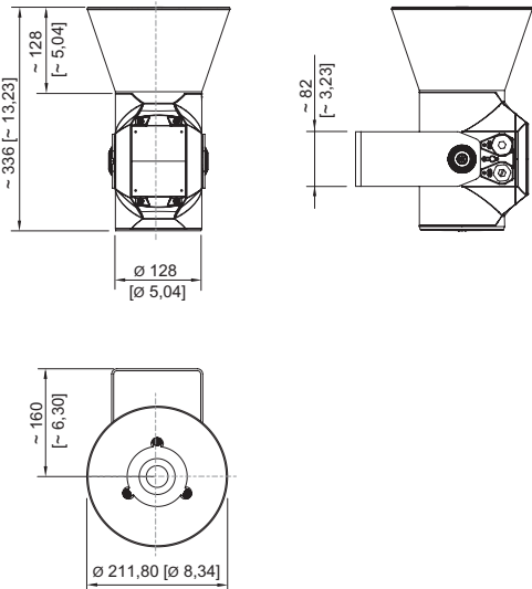
YA60/3 directional horn
