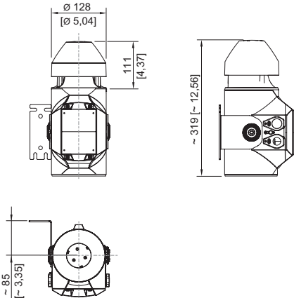
YA60/3 omnidirectional horn
