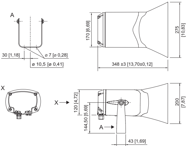
Hazardous area loudspeaker – long trumpet Bracket (A) supplied as standard
