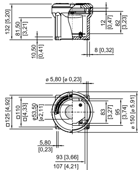
Size 1 enclosure with sight glass
