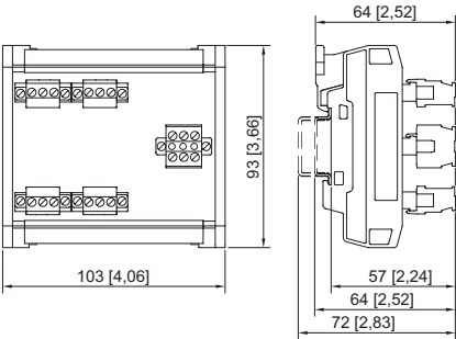
Field device coupler, 4 spurs, without enclosure
