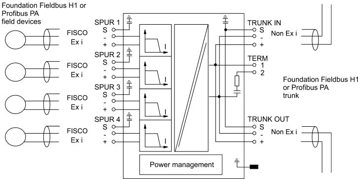
Connection diagram 9411/2.
