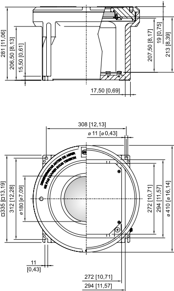
Size 6 enclosure with sight glass
