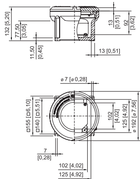
Size 2 enclosure without sight glass
