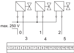
9477/12-08-12 connection diagram
