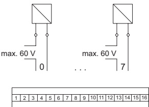
9477/12-08-12 connection diagram
