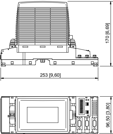
CPU & power module for Zone 1 with connection by means of Ex e terminals
