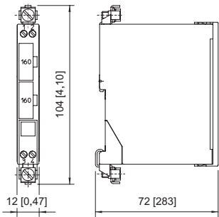
Single-Channel Safety Barriers with Electronic Current Limitation for Positive Polarity
