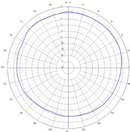
Radiation characteristics for 2.1 GHz Type 9790/1-0826-NTM-02
