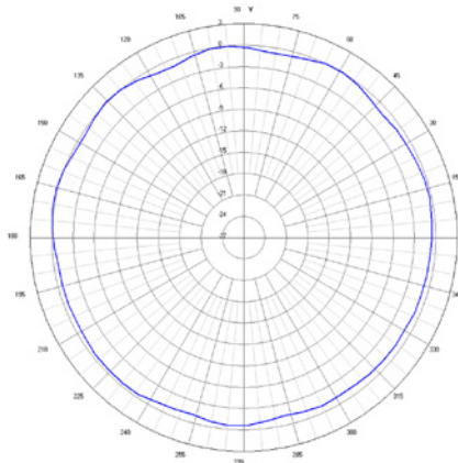
Radiation characteristics for 2.59 GHz Type 9790/1-0826-NTM-02
