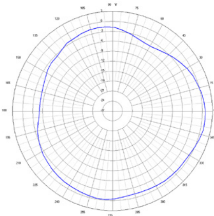
Radiation characteristics for 920 MHz Type 9790/1-0826-NTM-02
