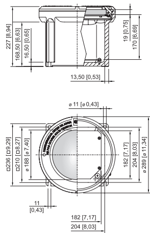
Size 4 enclosure with sight glass
