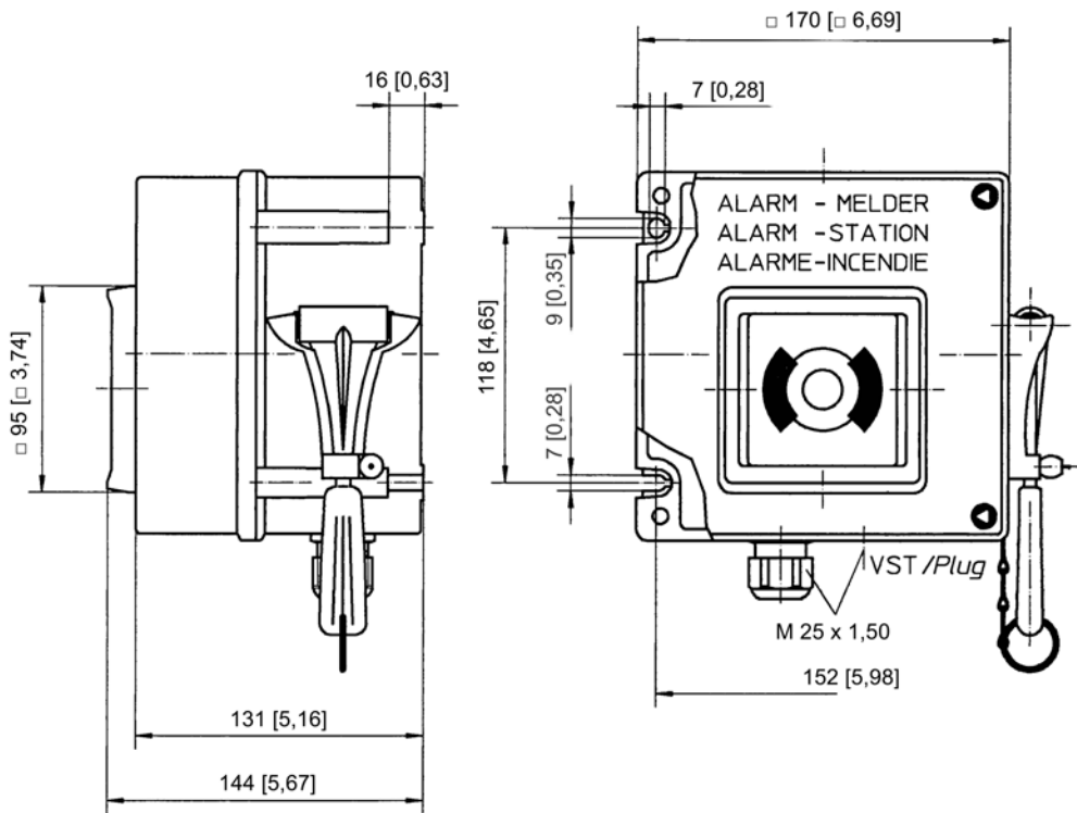
Dimensional Drawings (All Dimensions in mm [inches]) – Subject to Alterations
