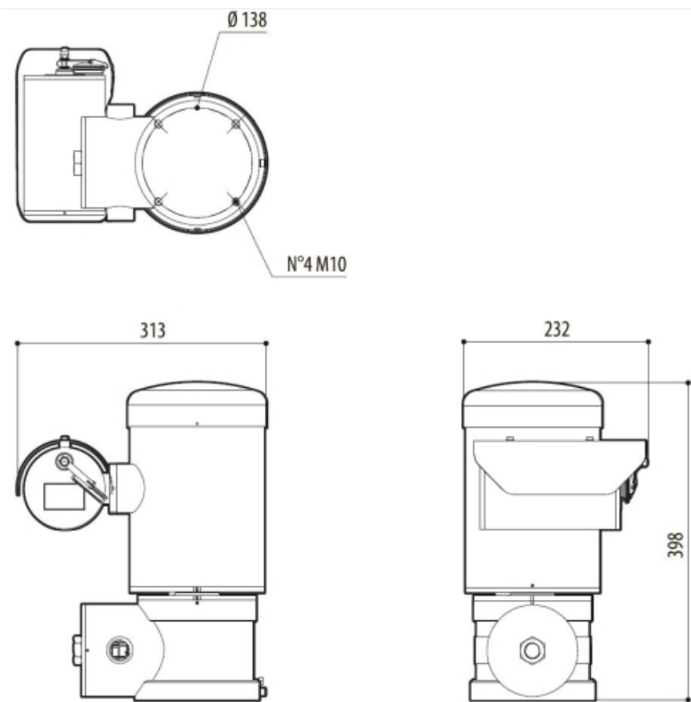
Dimensional Drawings (All Dimensions in mm [inches]) – Subject to Alterations
