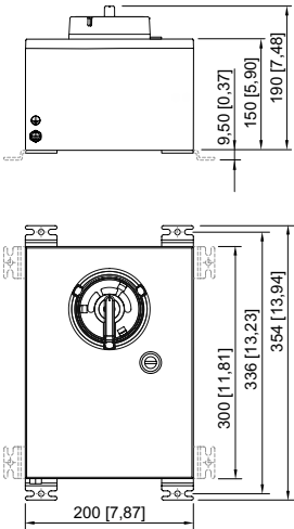
Dimensional Drawings (All Dimensions in mm [inches]) – Subject to Alterations
