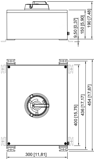
Switching arrangement 8544/1-3 and 8549/1-3
