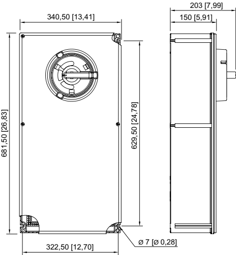
Dimensional Drawings (All Dimensions in mm [inches]) – Subject to Alterations
