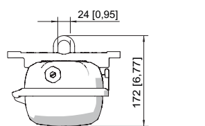
Mounting bracket fitted in mounting rail
