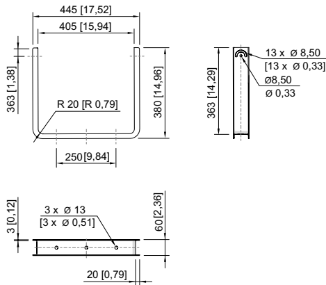
Mounting bracket
