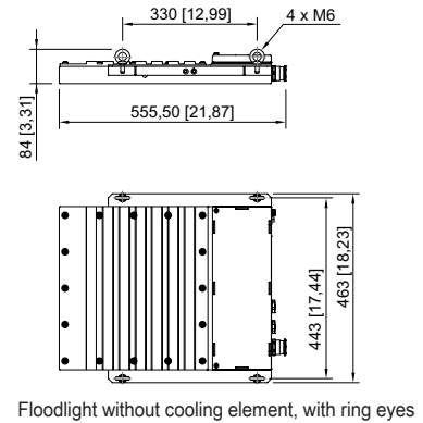
Floodlight without cooling element, with ring eyes
