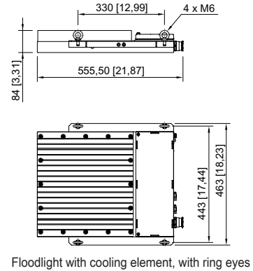
Floodlight with cooling element, with ring eyes
