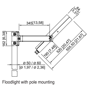
Floodlight with pole mounting
