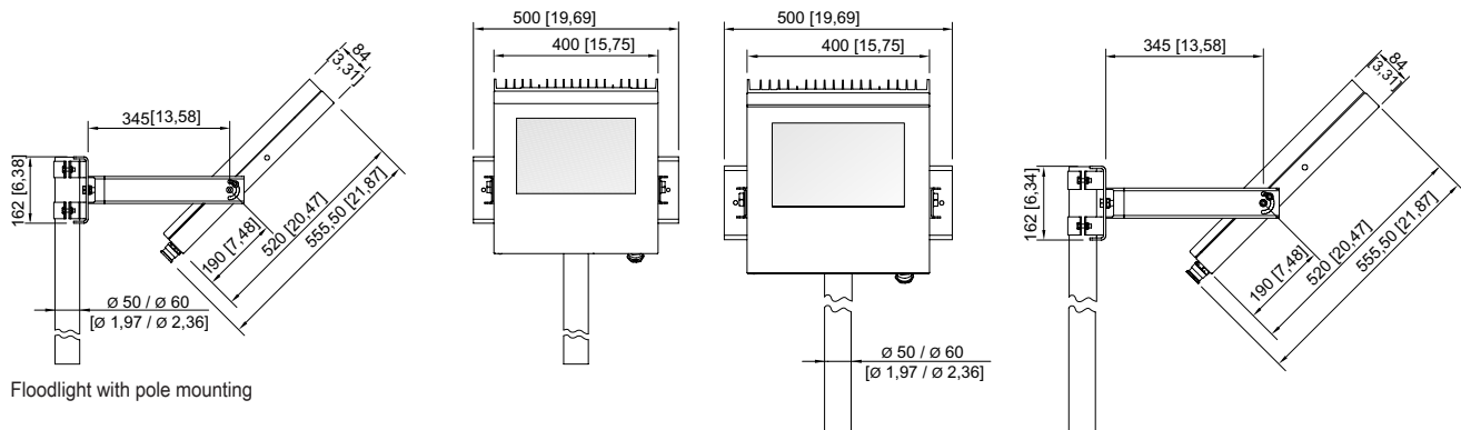
Mounting bracket
