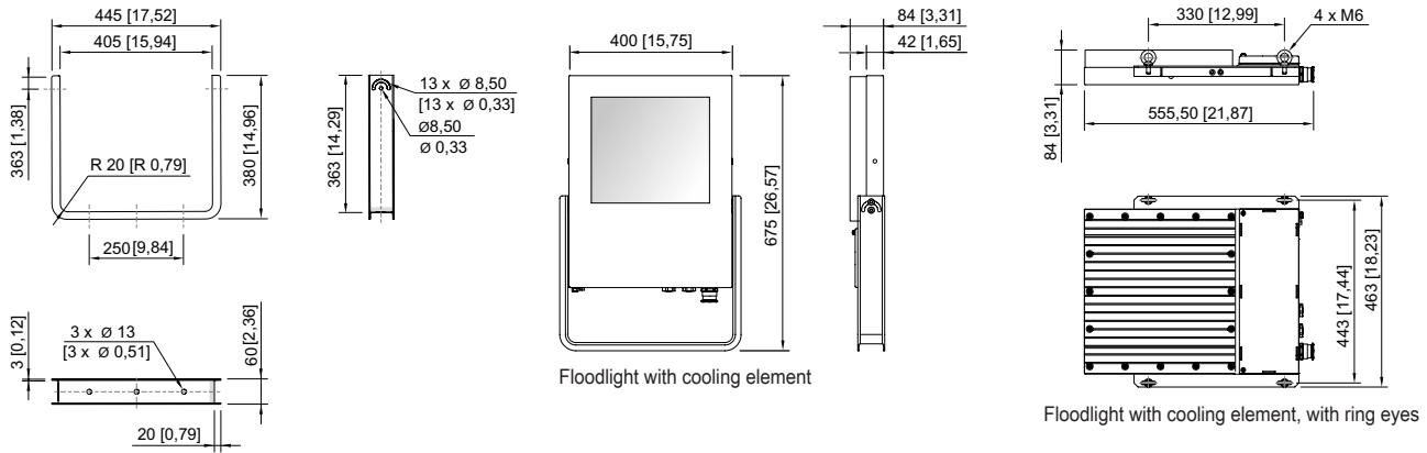
Mounting bracket
